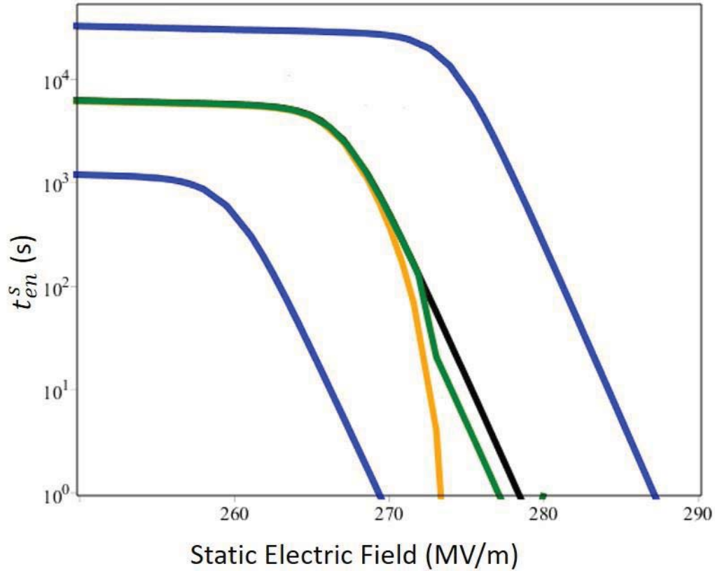
FIG. 5.6. Comparison of various SVET predictions. Traces include the prediction with no correction for the ramp up to the static waiting voltage (black), with the correction (green), and substituting the waiting voltage stress for the ramp-up voltages (yellow). The blue curves represent 5% variations in the black SVET prediction.
