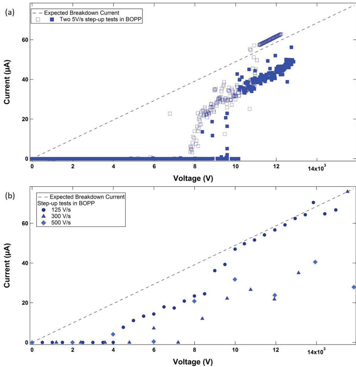
FIG. 4.8. Current traces from example voltage step-up tests in biaxially-oriented polypropylene (BOPP). Dashed lines correspond to Ohm's law for the circuit's current limiting resistors. (a) Plot of two step-up tests with \sim 5 \text{ V/s} ramp rate. In the test with the open markers, an area of erratic traces precedes the smooth ohmic slope. The test with solid markers does not transition to a smooth slope. (b) Plot of three step up tests at ramp rates of 125 \text{ V/s} , 300 \text{ V/s} , and 500 \text{ V/s} . In these cases, there is not a clear discontinuity from negligible current to current measurements increasing ohmically with applied voltage.
