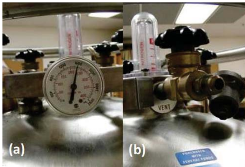
FIG. A.28. (a) LN_2 dewar pressure gauge reading ~250 psi. (b) LN_2 dewar vent/pressure release valve.
