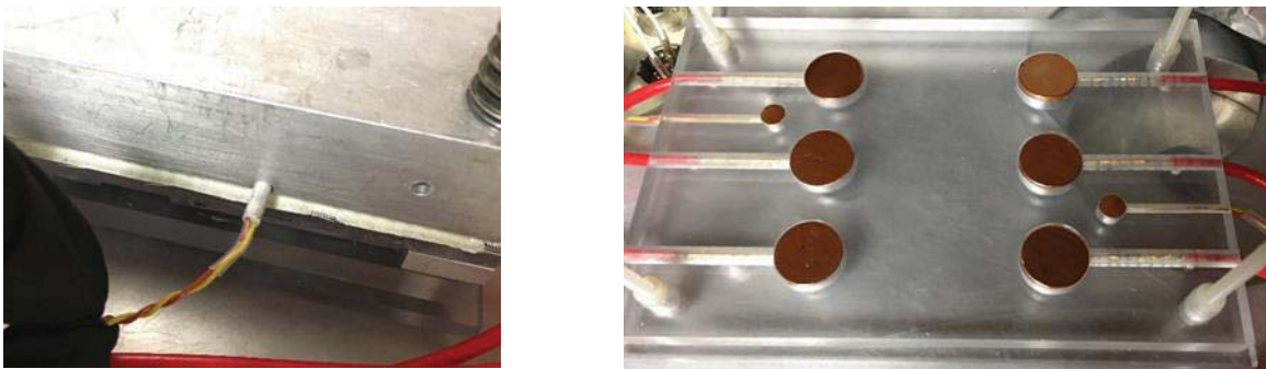
FIG. A.23. TC connections in the ESD chamber. Left- TC partially inserted into cryogenic reservoir. Right- TC electrodes circled in red on the ESD electrode plate.
