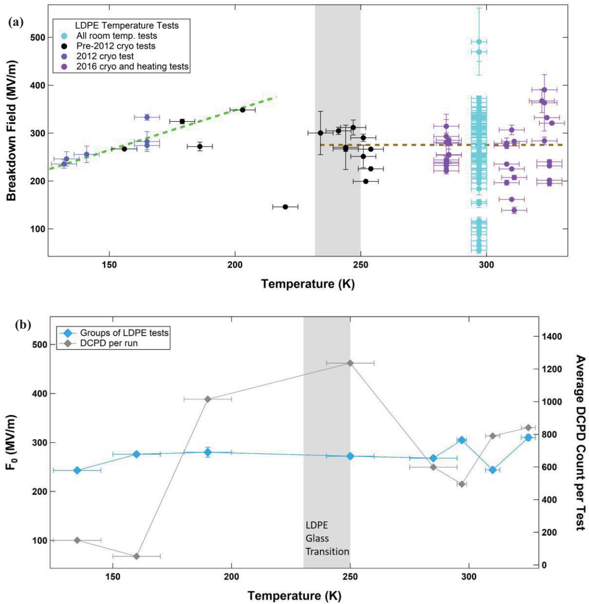
FIG. 6.4. Temperature effects on LDPE. (a) All LDPE standard ramp-up test data across temperatures from \sim 130 K to \sim 325 K. (b) Weibull scale parameter and average DCPD count for groups of tests of similar temperatures.
