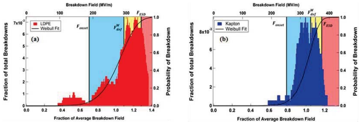
FIG. 5.9. Histograms of the fraction of total breakdowns versus breakdown electric field compared to the probability of breakdown at those fields given by Weibull distributions (black curves) for (a) 89 LDPE and (b) 36 Kapton (PI) step-up breakdown tests. F_{onset} to F_0 defines the blue region, F_0 to F_{ESD} defines the yellow region, and the red region is defined as field values above F_{ESD} .
