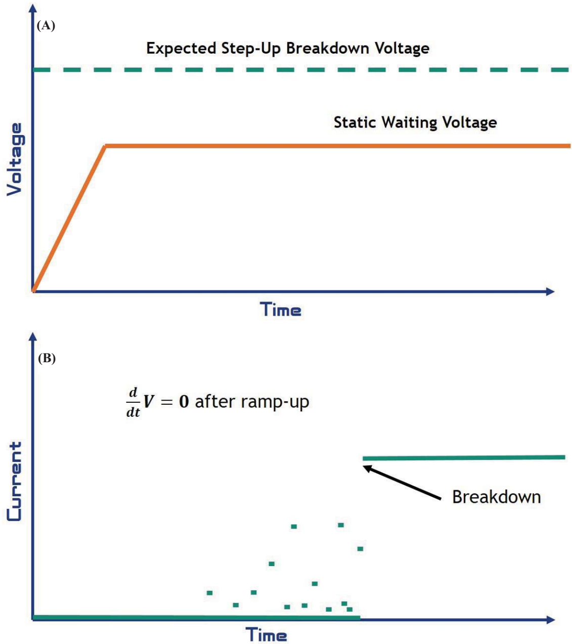
FIG. 4.3. Static Voltage Endurance Time (SVET) test method. (A) The applied voltage increases over time until the waiting voltage is achieved. The static waiting voltage is maintained for the duration of the test. (B) Current is measured throughout the test. Breakdown is marked by a transition to a large, constant, current set by the residual resistance of the test circuit.
